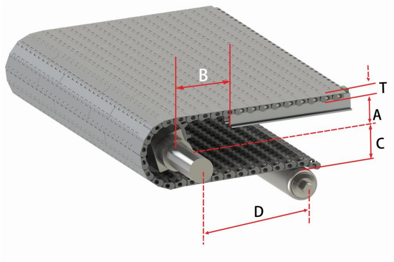
Conveyor Frame Dimensions
