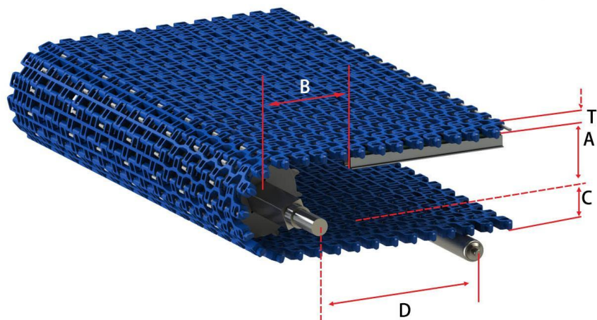
Conveyor Frame Dimensions
