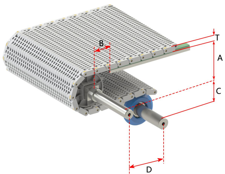
Conveyor Frame Dimensions
